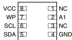
8-lead Leadless Array Bottom View
