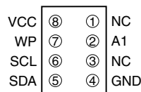
8-ball dBGA Bottom View
