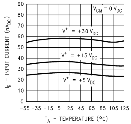
Input Current
